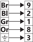
DHW valve V4043H
