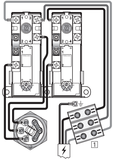
Electrical connection, diagram 2- 300-1000 I. UK WIRING- 7.5 kW - 3x400V
