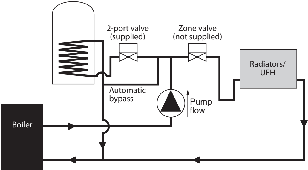
S-plan piping diagram
